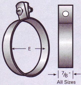
Tube Hanger
