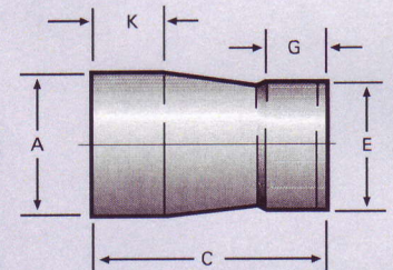
Standard Reducing Coupling (expanded end)
